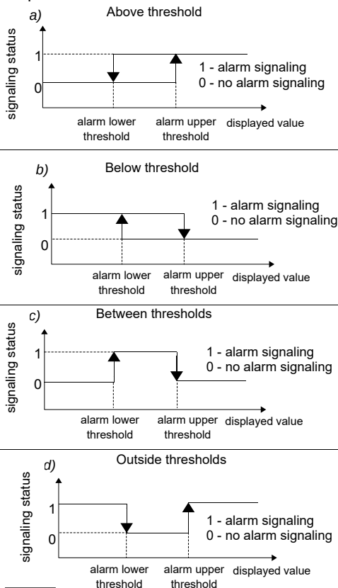
Fig. 11. Alarm types
