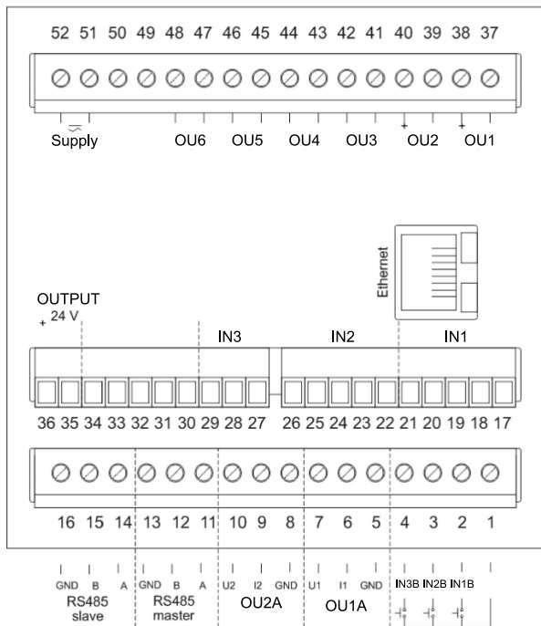
Fig. 3. Connection strips of the controller.
