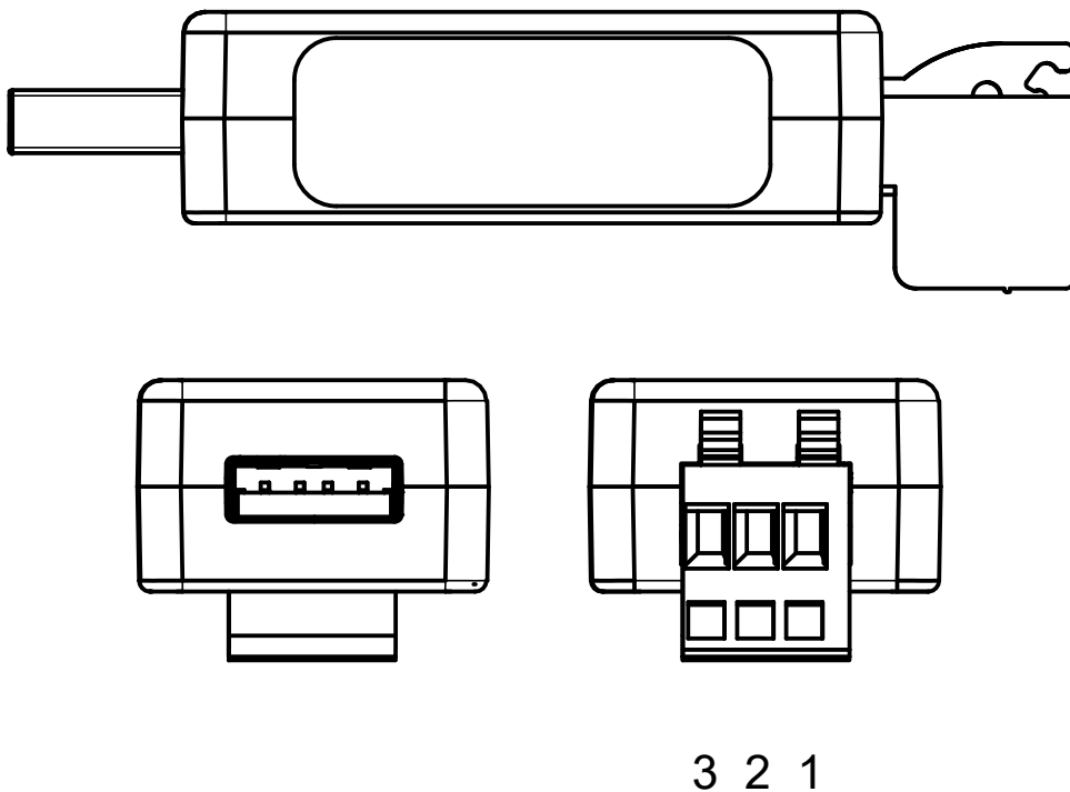
Fig. 3. PD20 converter pinouts.
