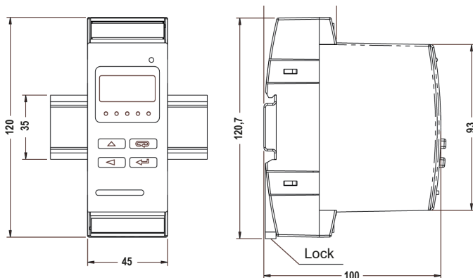
Fig. 2 Overall dimensions and mounting of the transducer.
