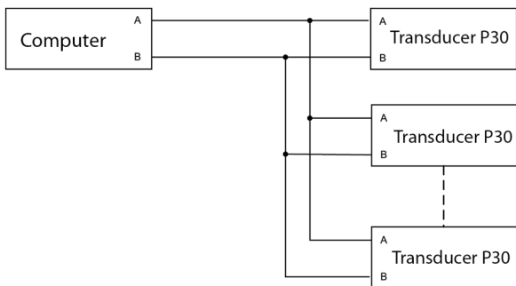
Fig. 21 Connecting the RS-485 interface.
