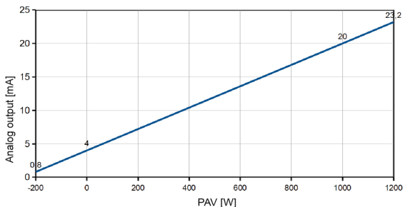
Fig. 10 Analog output with overrun support off
