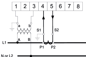
Fig.3 Wiring diagram of the P30P transducer
