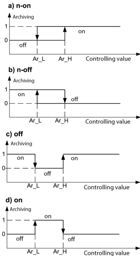
Fig. 18 Conditional archiving types
