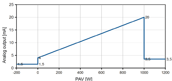
Fig. 11 Analog output with threshold limit handling on
