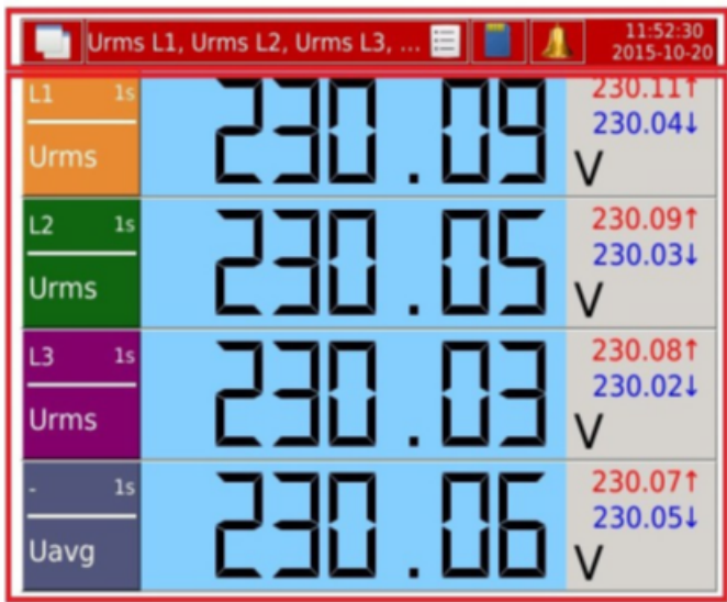
Fig. 23. Information elements.
