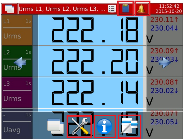
Fig. 22. Functional elements.
