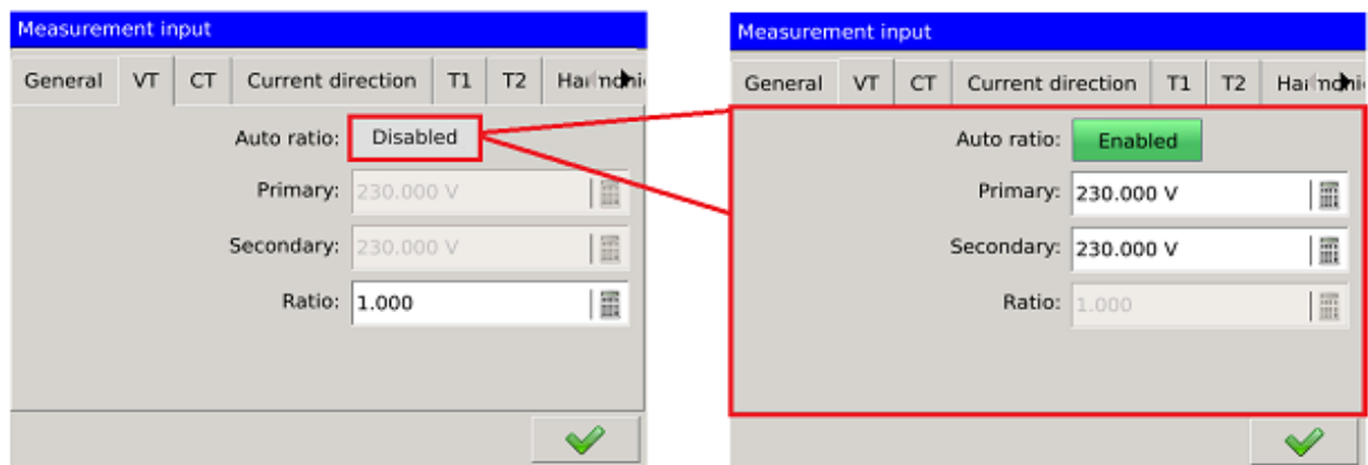
Fig. 104. Measurement input - voltage transformer ratio.
