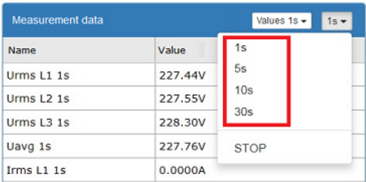
Fig. 80. Web server - change of refresh interval.
