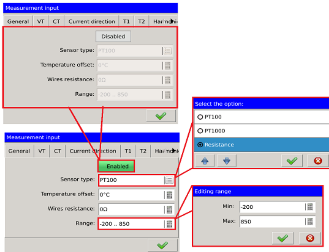
Fig. 107. Measurement input - temperature/resistance.
