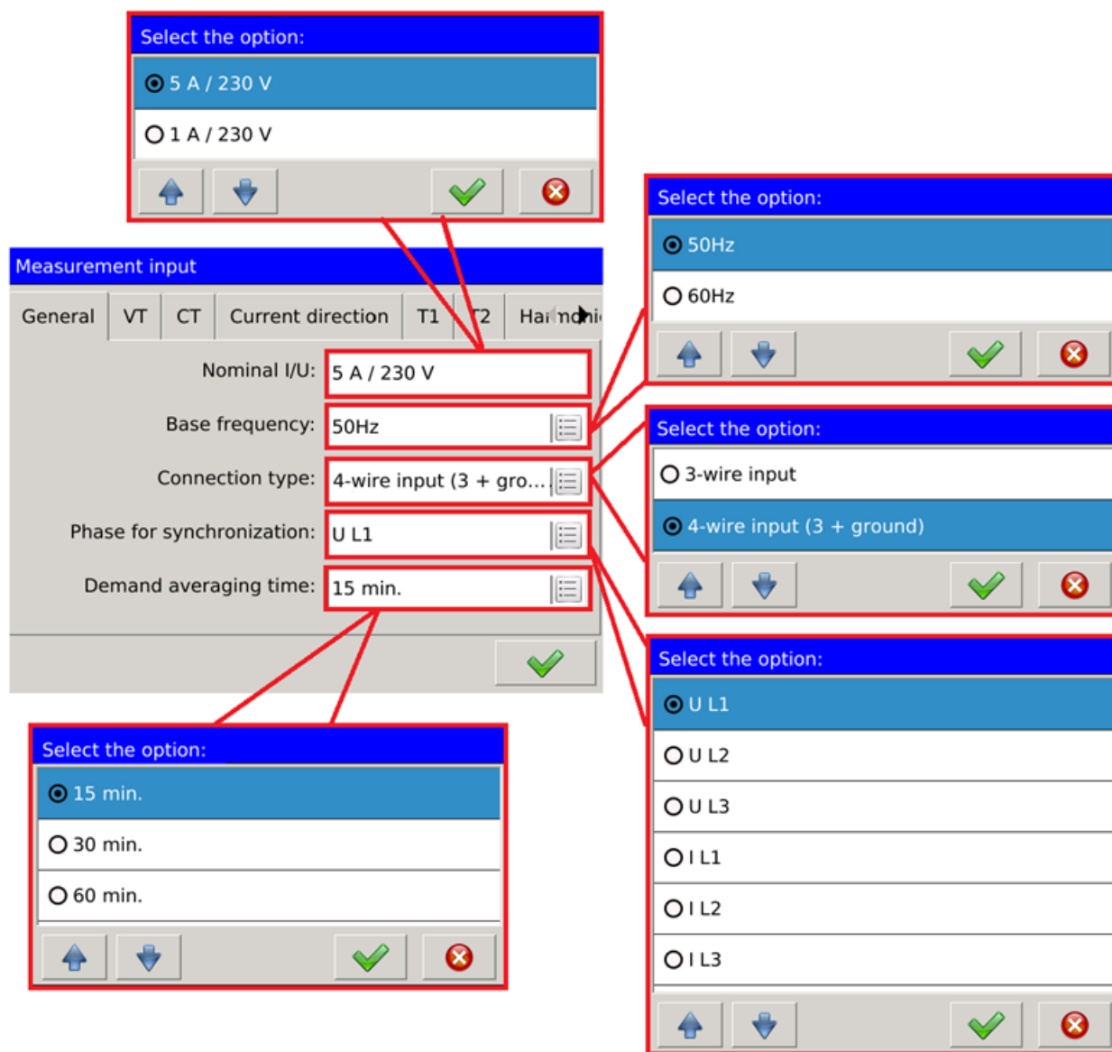
Fig. 103. Measurement inputs - general settings.
