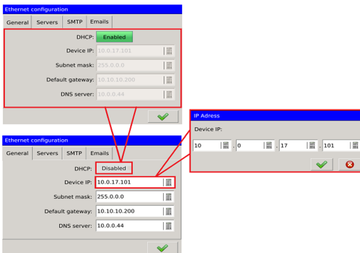
Fig. 116. Ethernet - general settings.
