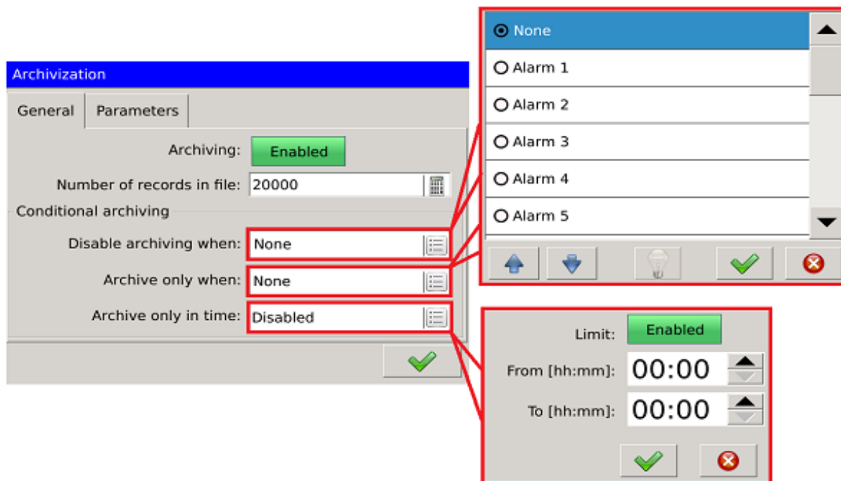
Fig. 122. Archiving - general settings.
