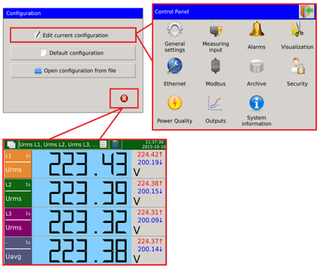
Fig. 36. Navigation - Control Panel.
