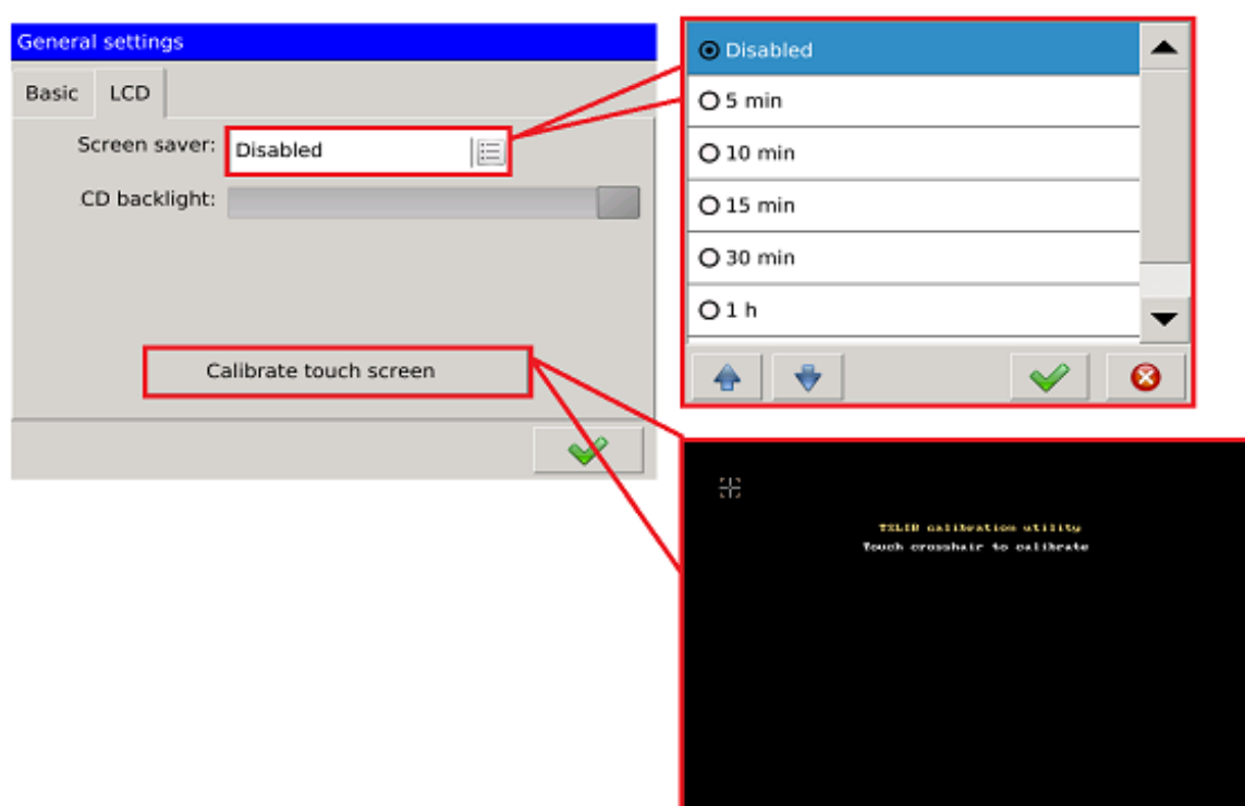
Fig. 102. General settings - LCD.
