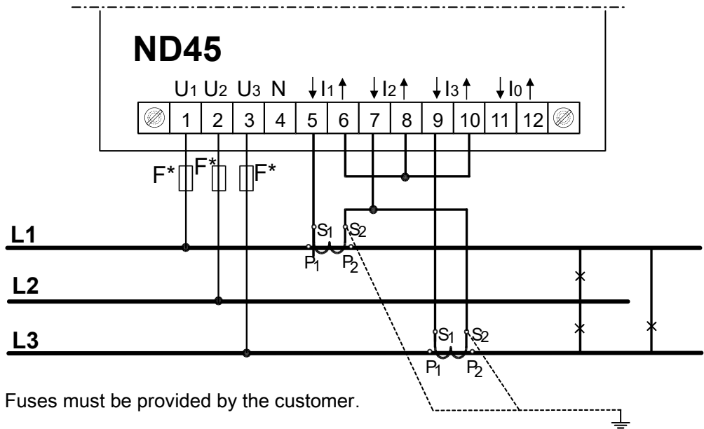
Fig. 3. Diagram - 3-wire network.
