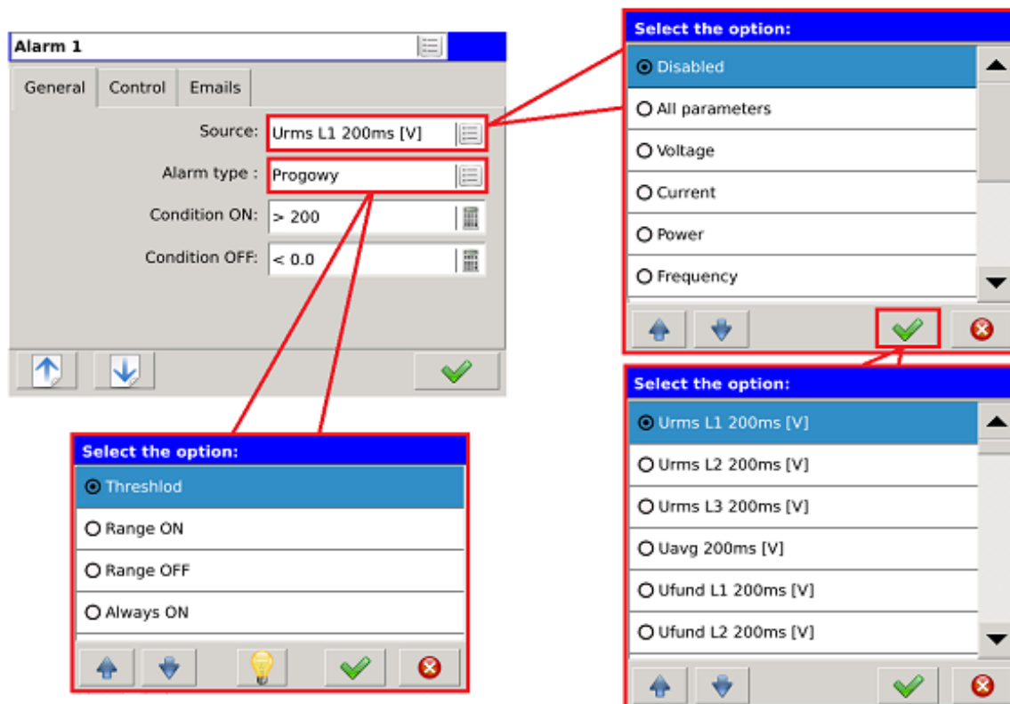
Fig. 110. Alarms - general settings.
