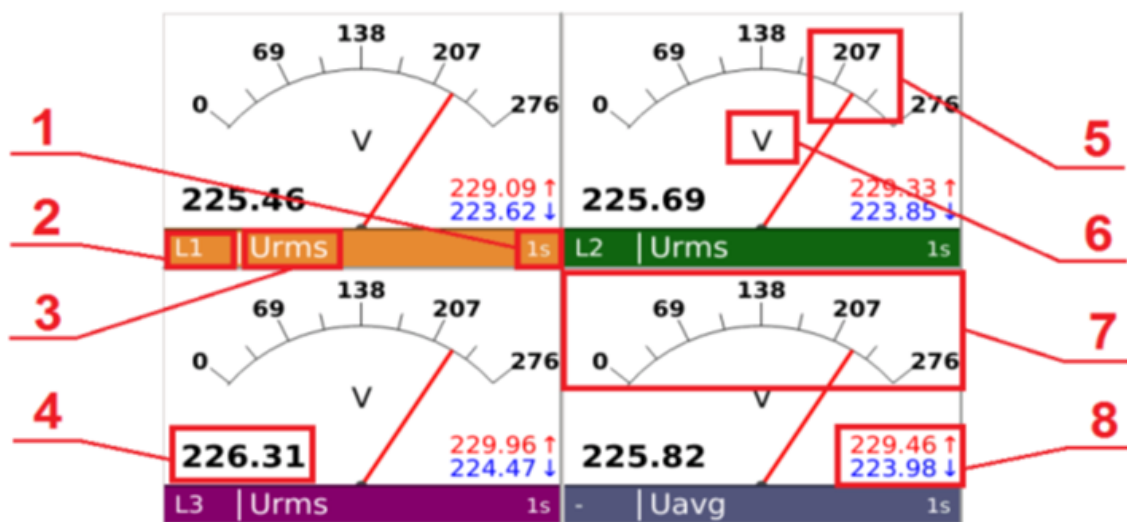
Fig. 57. Analog indicators.
