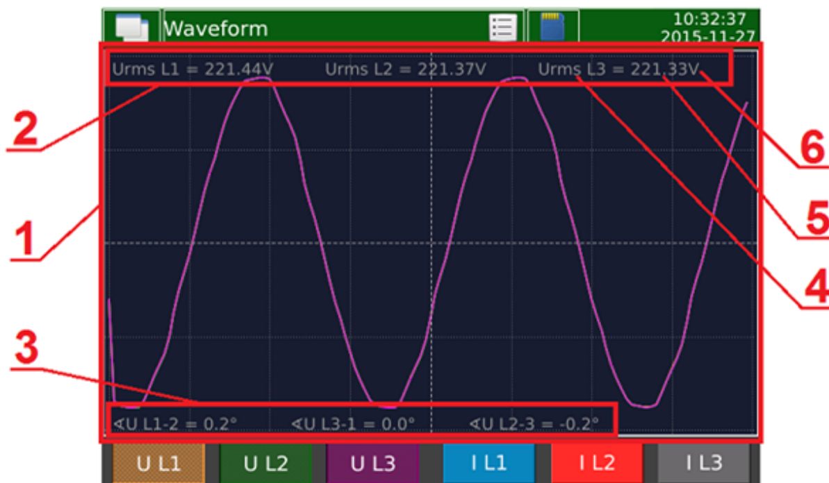
Fig. 63. Waveform.
