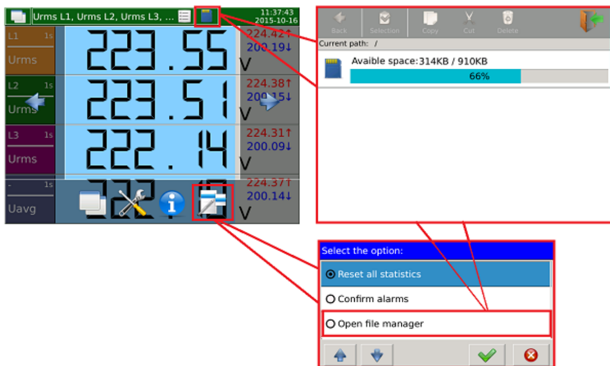
Fig. 137. File manager – navigation.
