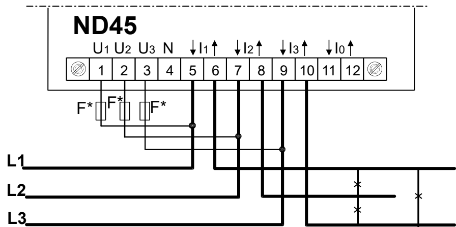
Fig. 2. Diagram - 3-wire network.
