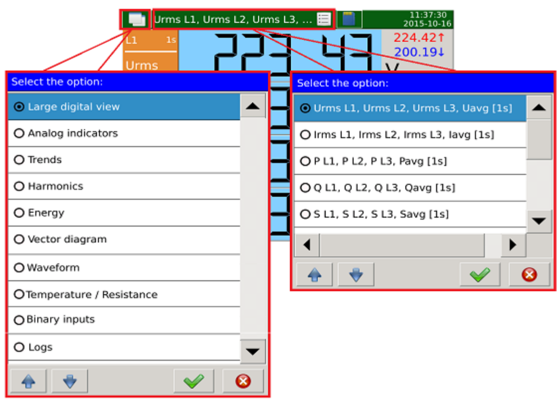
Fig. 27. Navigation - switching views and screen.
