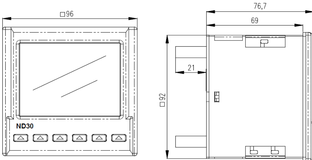
Fig. 3. Overall dimensions of the ND30 meter
