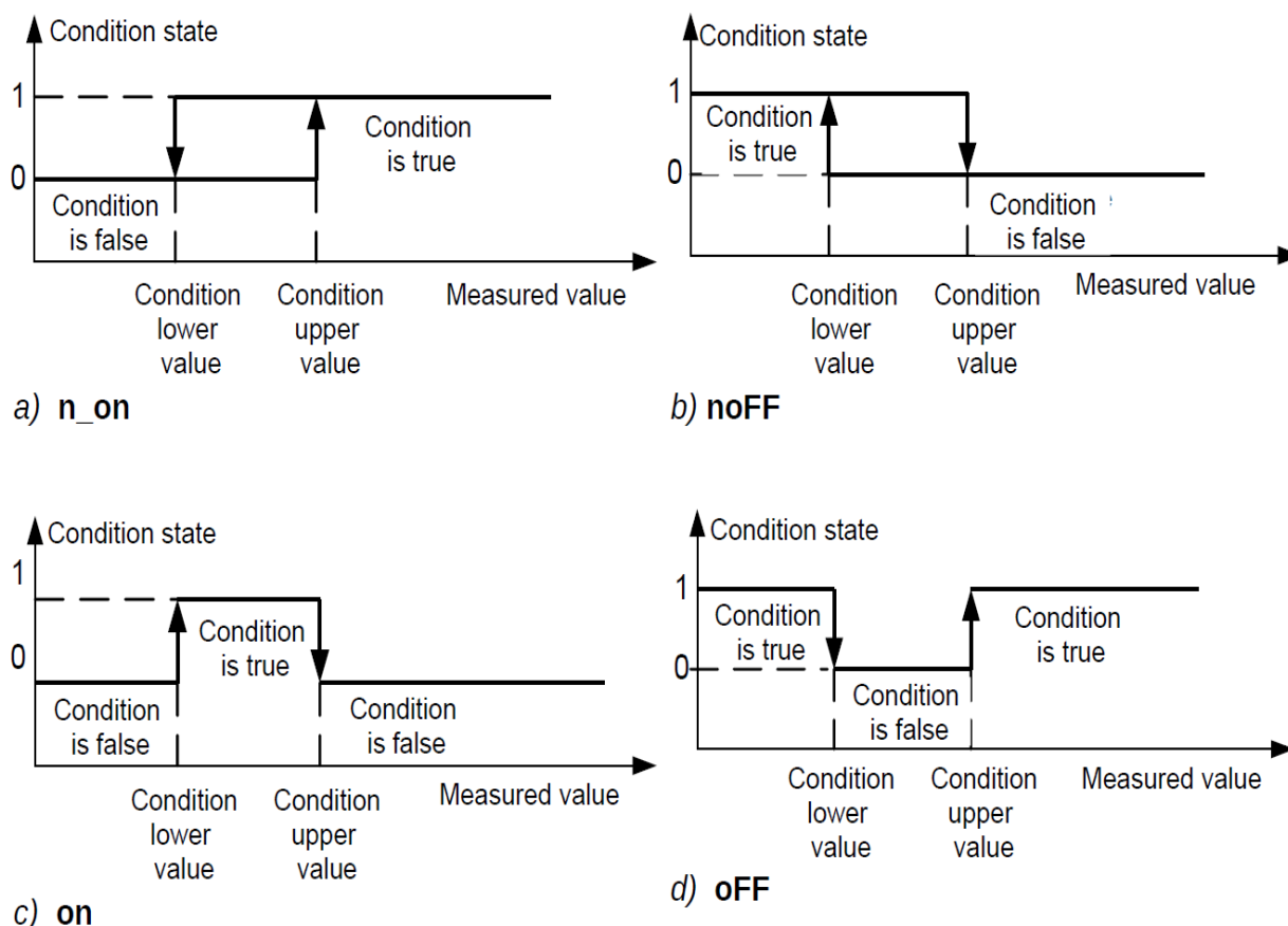
Fig. 17. Condition types: a) n_on b) noFF c) on d) OFF
