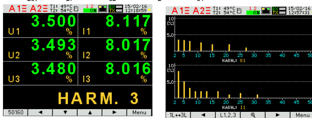
Fig. 13. Screens 11 and 12 - visualization of harmonics
