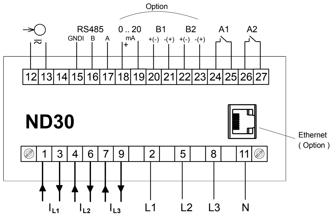
Fig. 4. Meter connections
