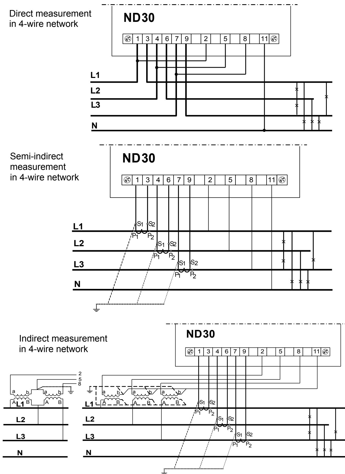
Fig. 6. Meter connections of input signals in a 3-phase 4-wire network
