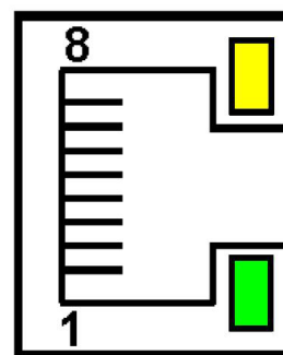
Fig. 28. View and pin numbering of the RJ45 socket
